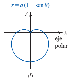
FIGURA 10.5.6 Cardioides
